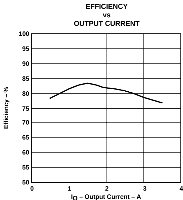
Figure 2–2. Measured Efficiency
