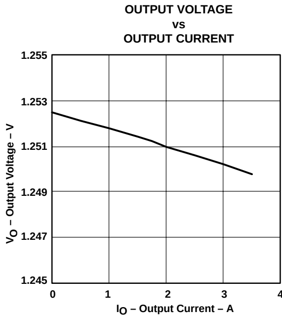
Figure 2–4. Load Regulation
